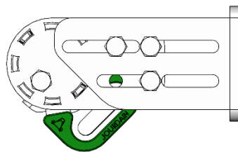
Montage / Mounting 45°
