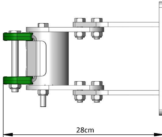
Montage / Mounting maxi
