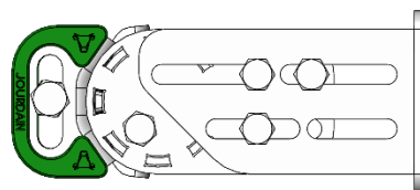
Montage / Mounting 180°
