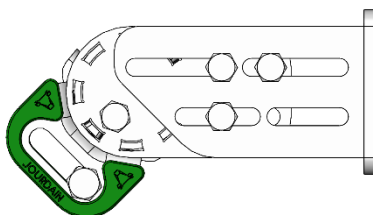
Montage / Mounting 135°
